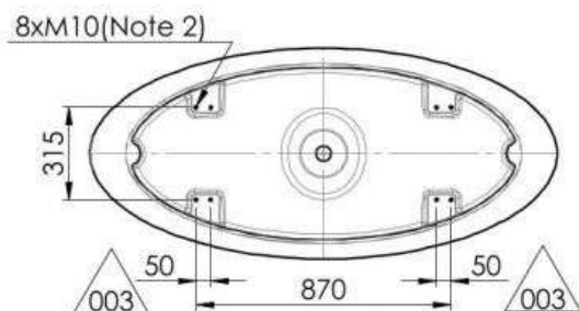
Bottom view
