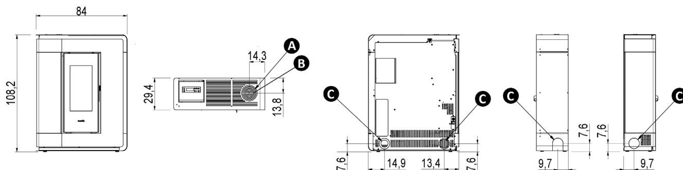
Fig. 18 - Arco 7/9 Bi-Flux
